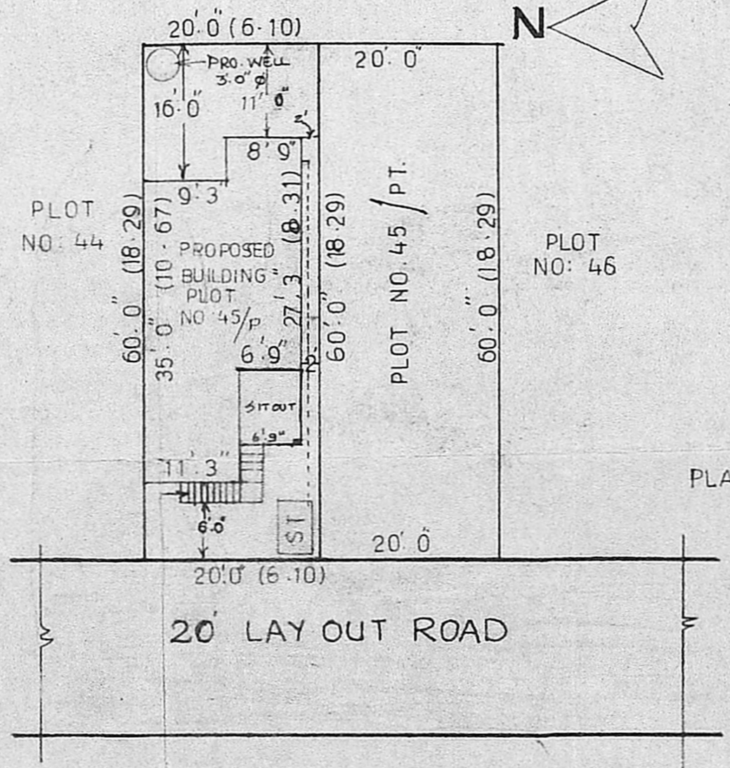
SITE PLAN
